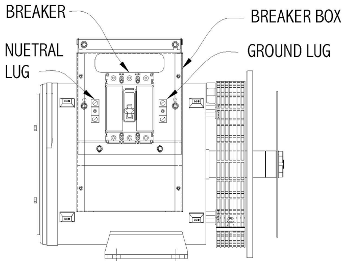
BREAKER BOX MAY BE MOUNTED ON EITHER SIDE OF ALTERNATOR 280 FRAME SIDE VIEW
